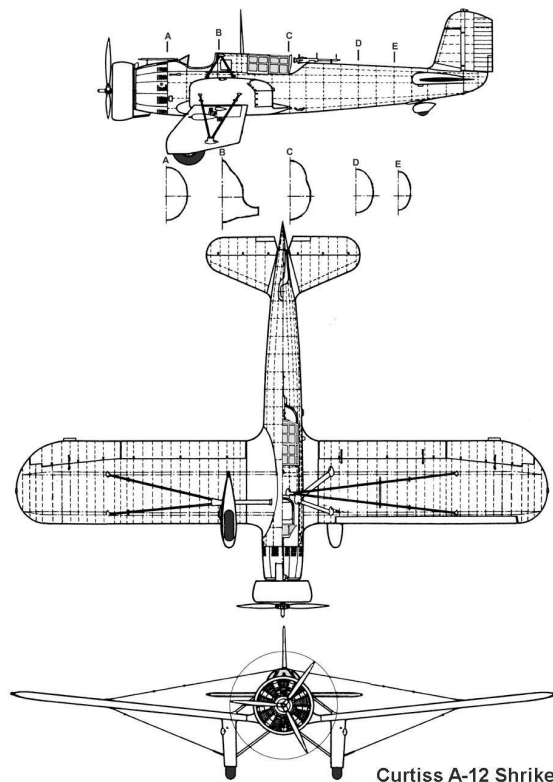
Curtiss A-12 Shrike
